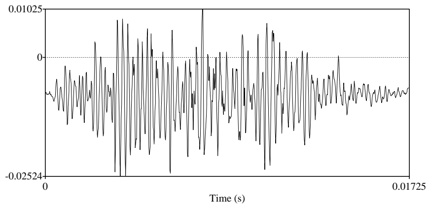
Figure 3: Waveforms of oral "ch" sound for a head approaching a flat computer monitor from a distance of 45 cm and 25 cm respectively.
