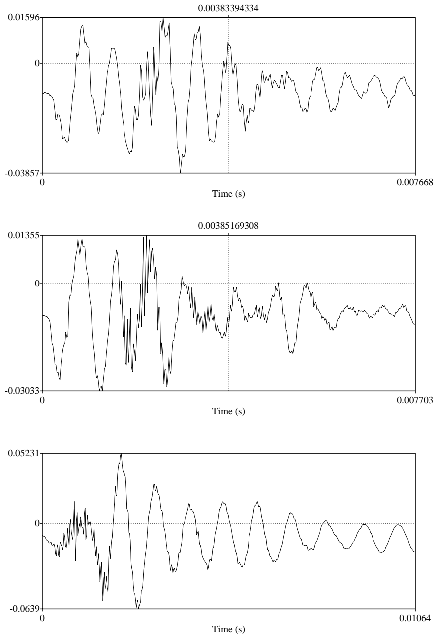
Figure 9: Three pulses of a sequence of palatal clicks for a head approaching a flat computer monitor from distances of 45, 25 and 5 cm respectively.
